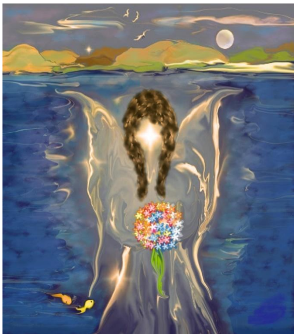
Figure 2: My imagination of water angel
