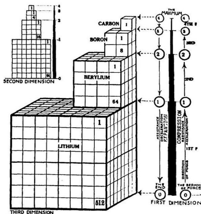
Figure 7: All demnsions are based upon tonal relations in octave wave fields
