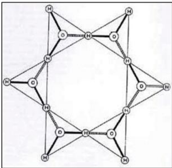
Figure 3: Geometry of the water entity
