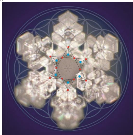
Figure 3: This figure explains water hexagonal structure better than any words
