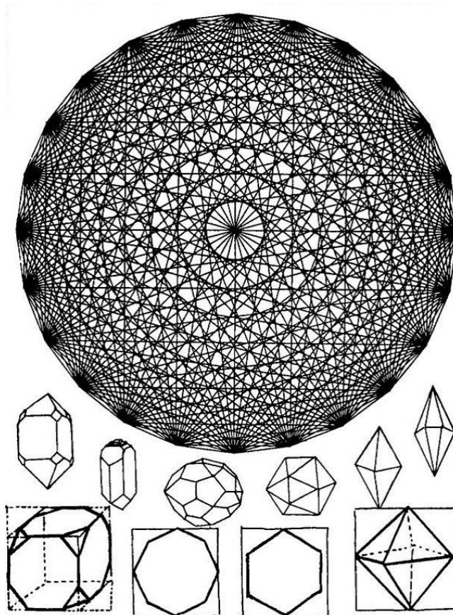
Figure 8: All forms of all bodies are based uopn the cube-sphere and its intersections
