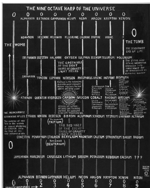
Figure 10: The Walter Russell Chart of the Elements of Matter
