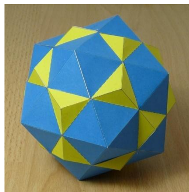
Figure 1: Dodecahedron into Icosahedron
