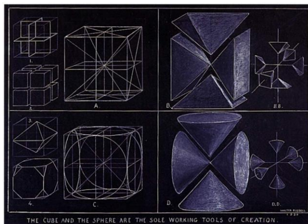
Figure 6: This diagram illustrates the manner in which the cube controls the curved universe of motion from its static condition. Within its tetrahedrons, its spirals revolve as cones as in two of them while in the central four, the spirals revolve within one plane to create the gravity fields which are known as magnetic fields
