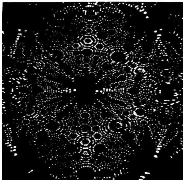
Figure 12: Photomicrograph of a pure tungsten crystal magnified 2,700,000 times, which was made by Cenco-Muller Ion Filed Microscope. The hexagonal form of water crystals is clearly shown in this picture
