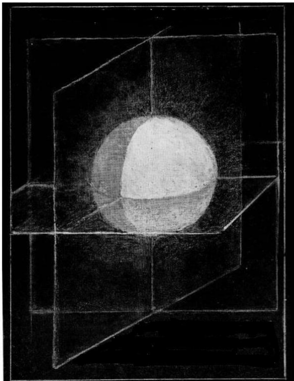
Figure 9: This diagram represents the radar intercommunication system of Nature. Its purpose is to tell everything in the universe what is happening everywhere else in the universe. There is nothing more powerful to demonstrate UNIVERSAL ONENESS than this diagram of the intercommunication system of Nature.
