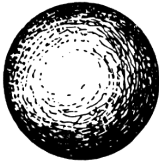
Figure 2.14: The sphere
