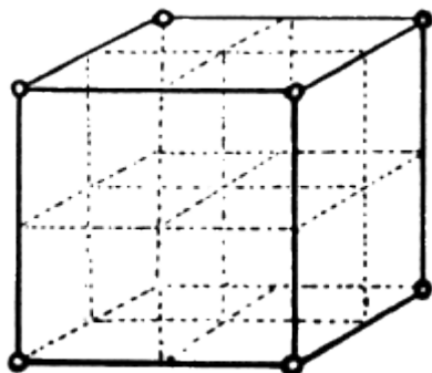
Figure 2.5: Mirror planes of reaction
