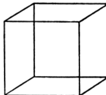
Figure 2.13: The cube
