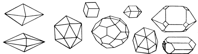
Figure 2.15: All crystals are cube sections
