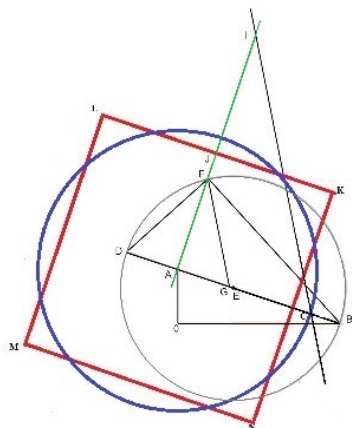
Figure 3.1: The geometric illustration of squaring the circle
