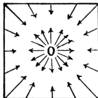
Figure 2.8: Sequential reactions
