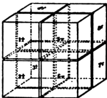
Figure 2.11: Repeated explosions compress
