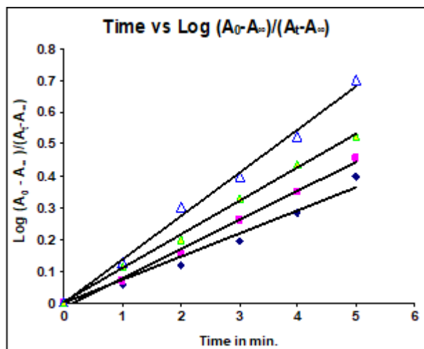
Figure 3(b): Plot of \log (A_0 - A_\infty) / (A_t - A_\infty) against Time For Hydrolysis of 5-Methyl salicylidene – m- methyl aniline
