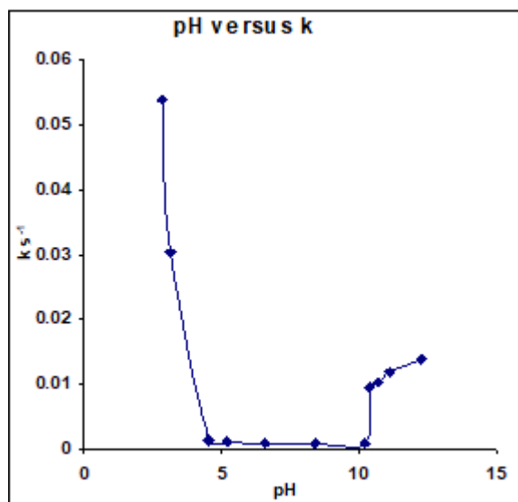
Figure 1: Plot of k against pH at 303 K for the hydrolysis of 5-Methyl salicylidene - m - methyl aniline at \mu = 0.1 \text{ mol dm}^{-3}
