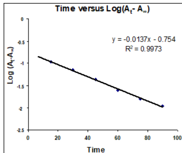
Figure 2(b): Plot of Time versus \text{Log} (A_t - A_\infty) at 30 °C for hydrolysis of 5-Methyl salicylidene – m-methyl aniline
