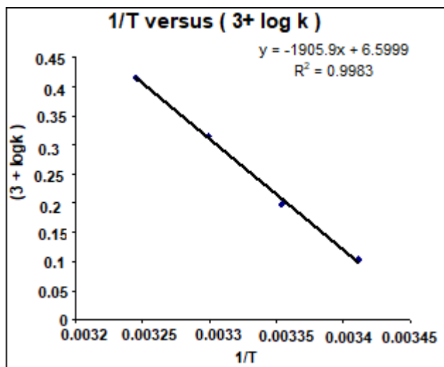
Figure 3 (a): Plot of (3 + \log k) against 1/T for hydrolysis of 5-Methyl salicylidene – m- methyl aniline
