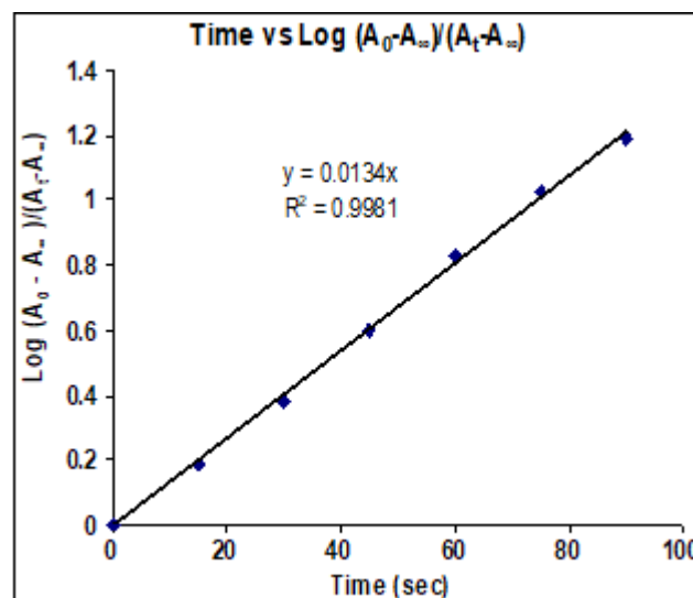
Figure 2(a): Plot of Time versus \text{Log} (A_0 - A_\infty) / (A_t - A_\infty) at 30 °C for hydrolysis of 5-Methyl salicylidene – m-methyl aniline at \text{pH} = 3.16
