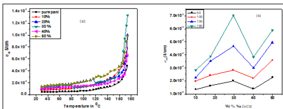
Figure 3: (a) shows the \sigma_{dc} conductivity as a function of temperature, (b) shows the variation of dc conductivity as a function of different weight percentages
