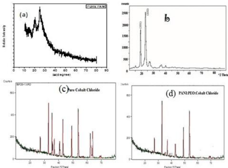
Figure 1: X-ray diffraction pattern of (a) Pure Polyaniline, (b) Pure PEO (c) CoCl 2 (d) 50wt% of CoCl 2 +PEO in polyaniline
