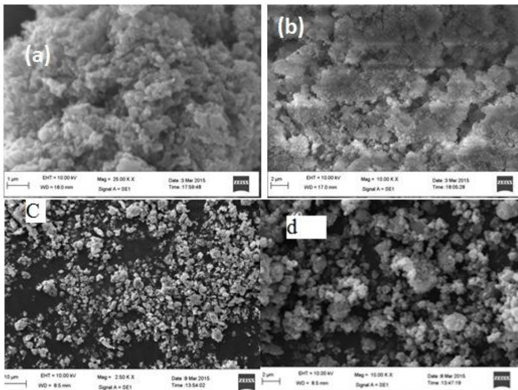
Figure 2: SEM image of (a) Pure polyaniline, (b) Pure PEO (c) Pure CoCl 2 (d) 50wt% of CoCl 2 +PEO in Polyaniline
