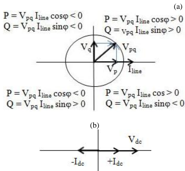
Figure 4: SSSC phasor diagram
