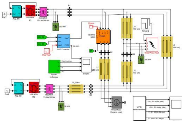
Figure 5: Static Synchronous Series Compensator (SSSC) used for power oscillation damping
