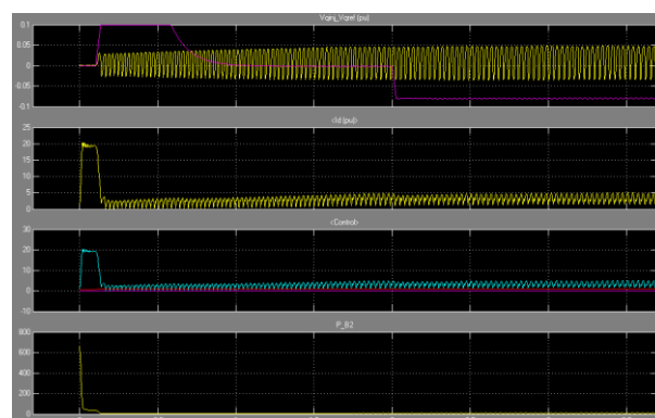
Case (b): LLL fault with POD controller
