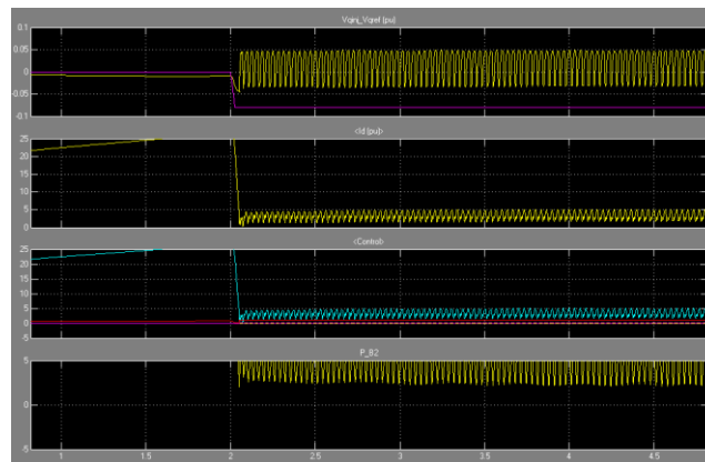
Figure 6 (a): Dynamic response of SSSC for LLL fault without POD controller
