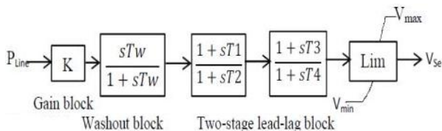
Figure 2: The structure of a simple FACTS POD controller
