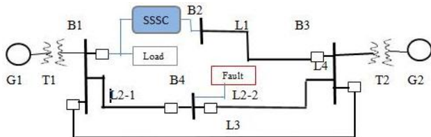
Figure 1: Single line diagram of a two-machine power system with SSSC
