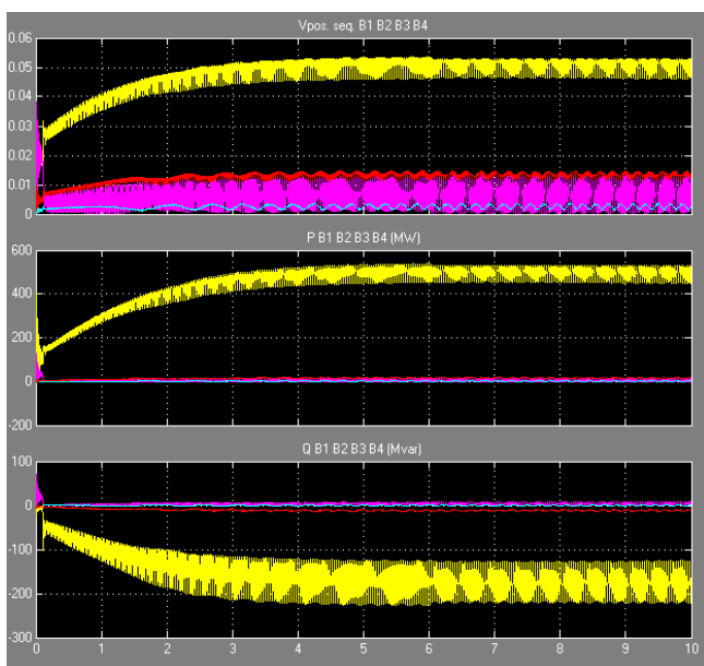
Figure 7(b): Simulated wave form for LLL fault with POD controller
