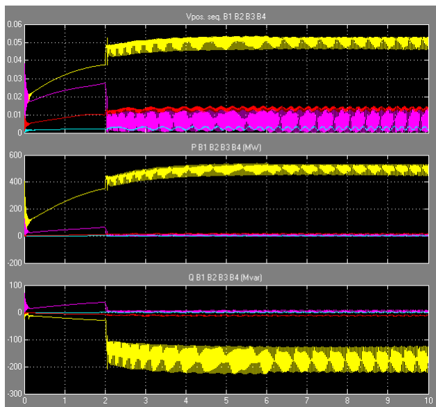
Figure 7(a): Simulated wave form for LLL fault without POD controller
