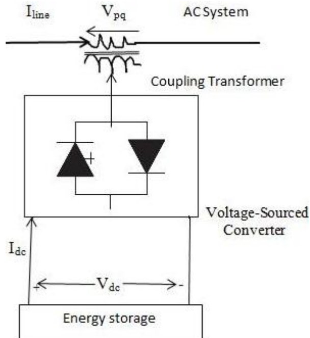
Figure 3: Functional model of SSSC
