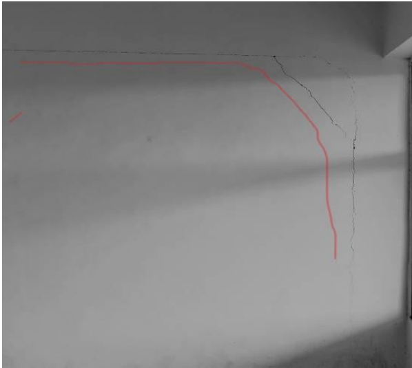
Photograph 7: Joint of column-wall and Beam-wall (Diagonal cracks)
