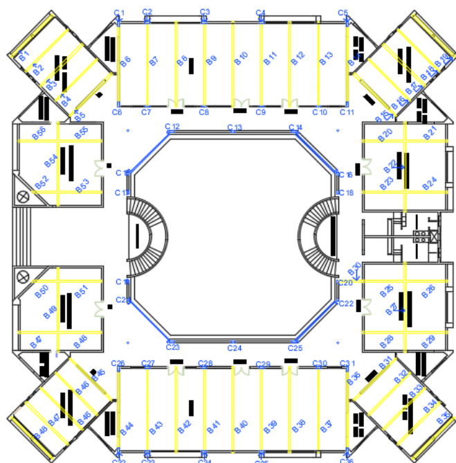
Figure 1: Plan of Building (JV)
