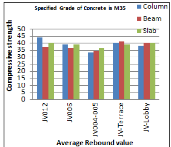
Figure 4: Graph of Rebound number v/s Compressive strength
