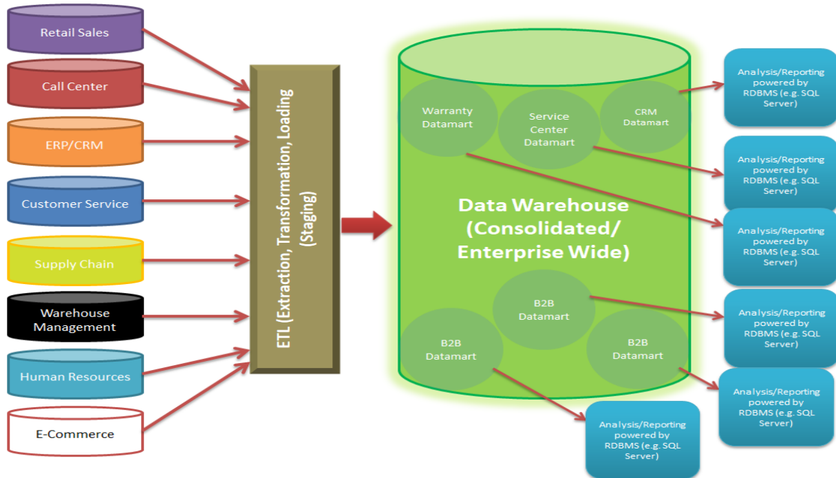
Big Data Activation: Data Warehouses and Data Lakes
