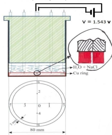
Figure 3: Experimental set-up
