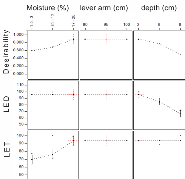
Figure 3: Effect of Moisture content, Lever arm length and Soil Depth on Soil Loosening Efficiency (LED and LET)
