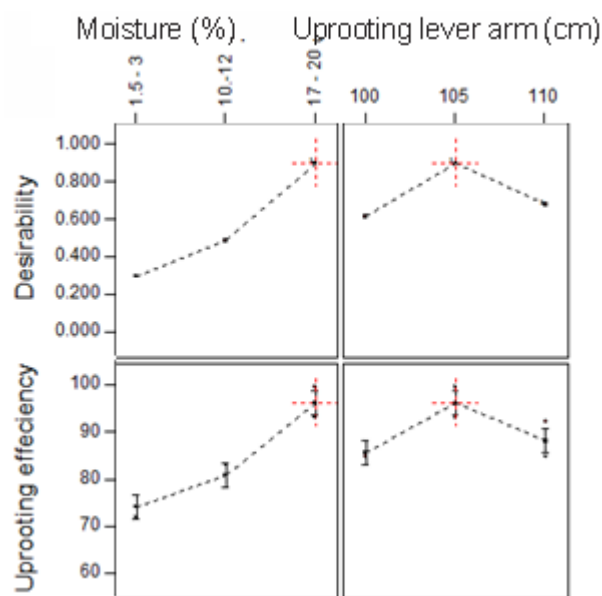
Figure 4: Effect of Uprooting Efficiency on Moisture and Length of Lever arm
