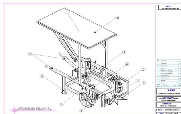
Figure 1: Push-Type Cassava Harvester
