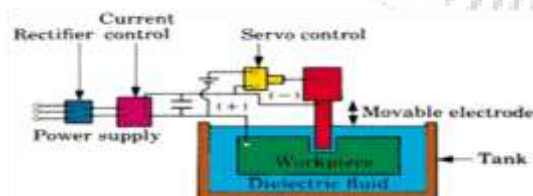
Figure 1: Schematic dig. Of EDM
