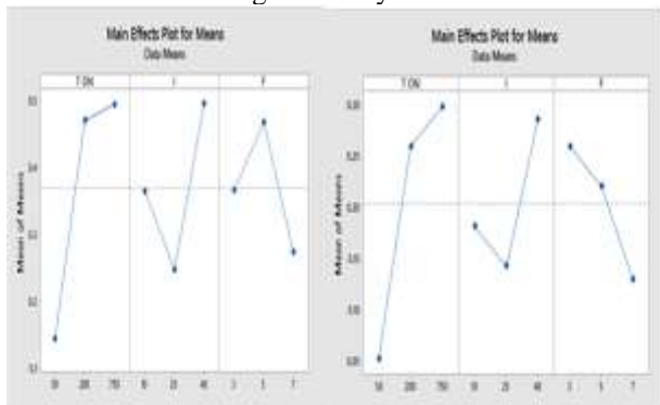
Figure 7: Means of means plot for copper and Brass
