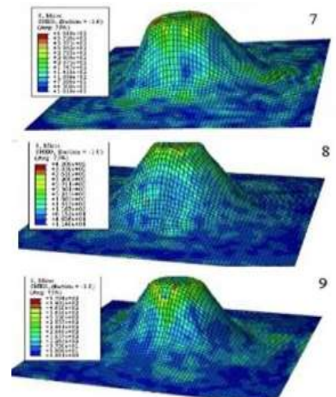
Figure 9: Equivalent stress induced in sheet thickness of 1.2 mm.
