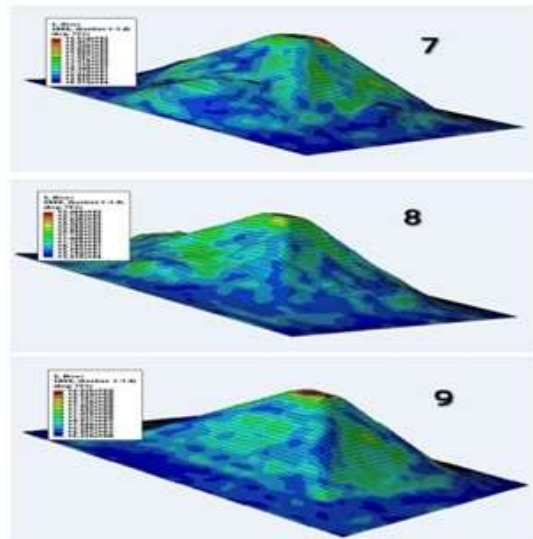
Figure 9: Equivalent stress induced in sheet thickness of 1.2 mm.
