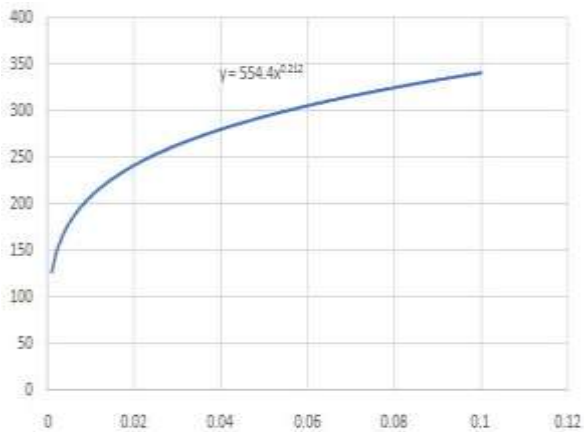
Figure 2: Load vs. Deflection of AA 5454 alloy.
