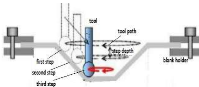
Figure 1: Single point incremental forming process.
