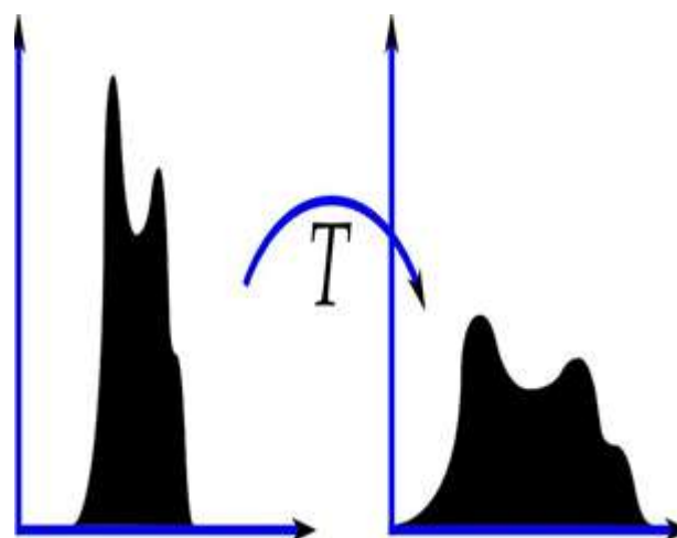
Figure 4: Histogram equalization
