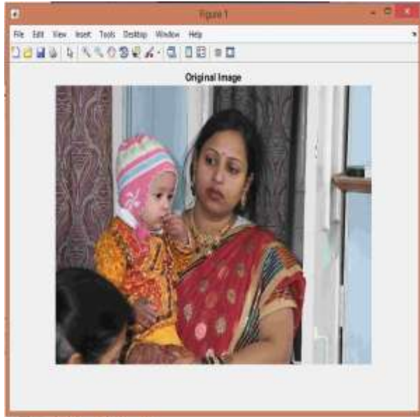
Figure 9: Original image
