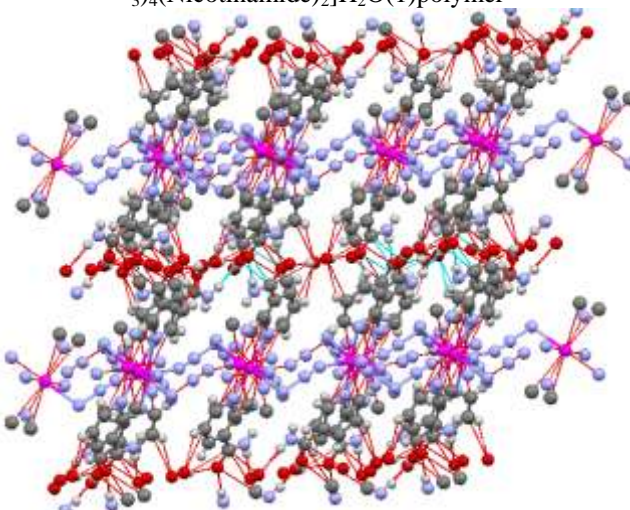
Figure 9: Perspective view of 3D structure of [\text{Cd}(\mu\text{-N}_3)_4(\text{Nicotinamide})_2]\text{H}_2\text{O}(1) polymer along the b axis
