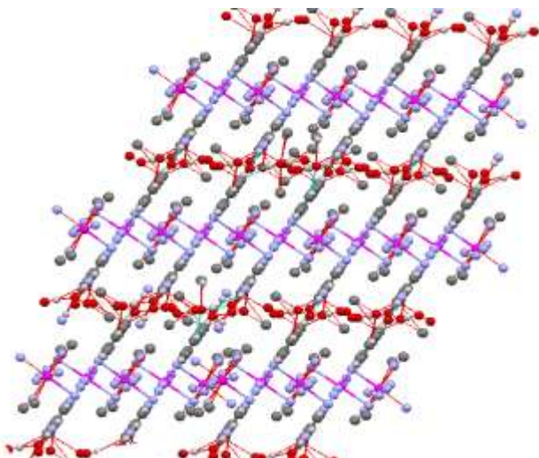
Figure 6: 2D grid like chain structure of [\text{Cd}(\mu\text{-N}_3)_4(\text{Nicotinamide})_2]\text{H}_2\text{O}(1) along the b axis
