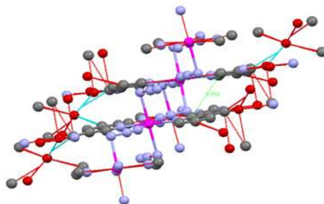
Figure 10: Shows distance between two pyridine ring along the b axis
