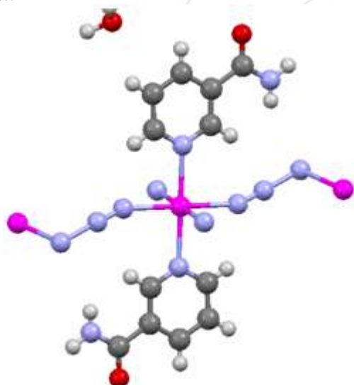
Figure 2: Ball and Stick model of single molecule of [\text{Cd}(\mu\text{-N}_3)_4(\text{Nicotinamide})_2] polymer(1)
