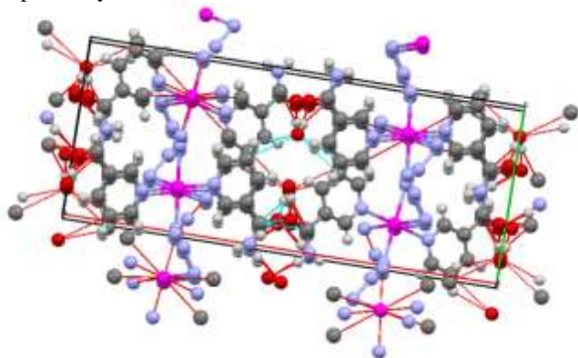
Figure 11: Packing Diagram of [Cd(\mu-N_3)_4(Nicotinamide)_2]H_2O polymer along the b axis
