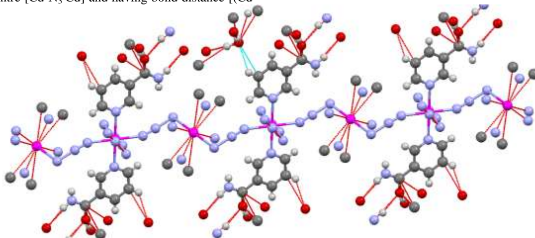
Figure 4: 1D chain of [Cd( \mu -N 3 ) 4 (Nicotinamide) 2 ]H 2 O( ) along the b axis (short contacts are shown in dotted red line)
