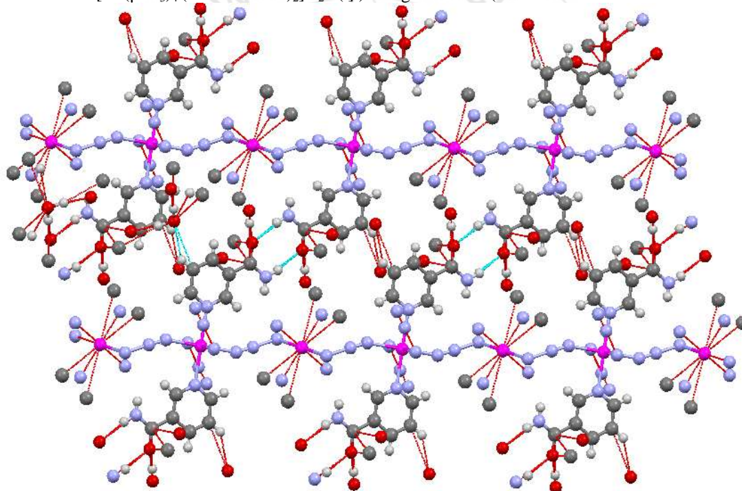
Figure 5: Hydrogen bonding between O(12)-H(12)--O(8) and N(9A)-H(9A)-O(8) which stabilise the 2D structure along the b axis
