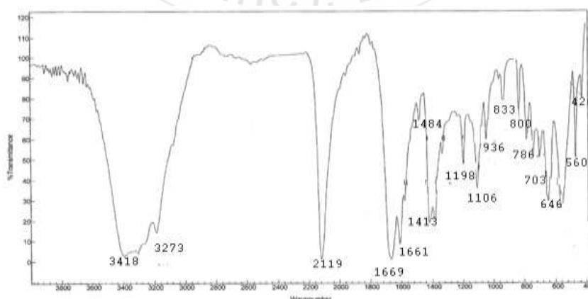
Figure 1: IR Spectrum of [\text{Cd}(\mu\text{-N}_3)_4(\text{Nicotinamide})_2]\text{H}_2\text{O}(1)
