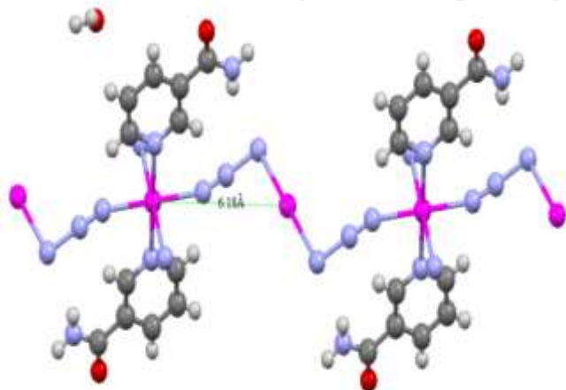
Figure 7: shows distance between Cd-Cd atoms of neighbouring molecule of [\text{Cd}(\mu\text{-N}_3)_4(\text{Nicotinamide})_2]\text{H}_2\text{O}(1) along the b axis
