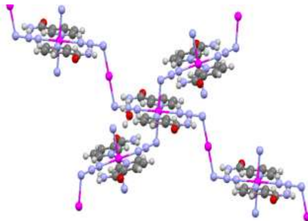
Figure 8: showing (\mu_{1,3}) bridging through azide along the a axis (central Cd ion bonded with four different Cd ion through bridging \text{N}_3^- anion ligand) in [\text{Cd}(\mu\text{-N}_3)_4(\text{Nicotinamide})_2]\text{H}_2\text{O}(1) polymer
