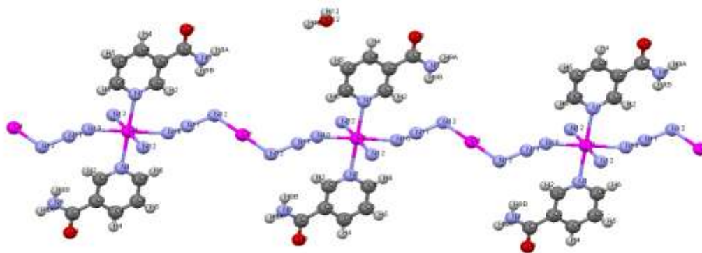
Figure 3: 1D chain of [\text{Cd}(\mu\text{-N}_3)_4(\text{Nicotinamide})_2] along the b axis for (1)
