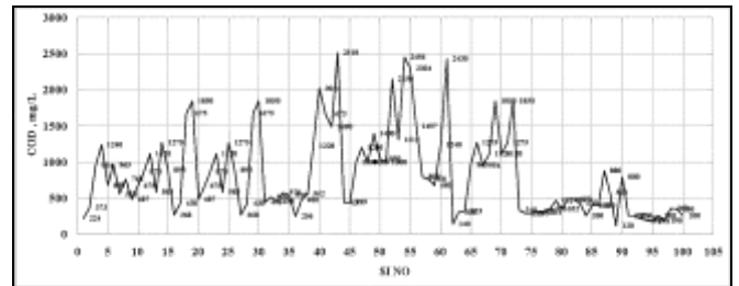
Figure 2: Distribution of chemical oxygen demand (COD) of the wastewaters for the hundred textile processing wastewaters.
