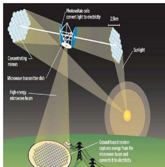
Figure 3: Shows a design of Space based Solar Power (SBSP)
