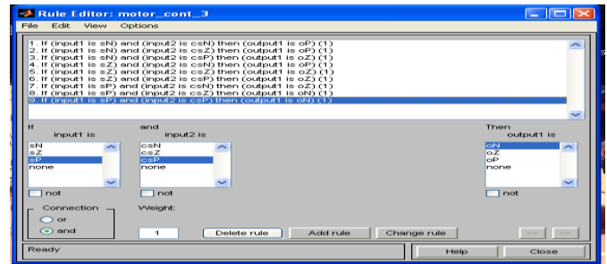
Figure 6: Fuzzy rules for 3 membership function
