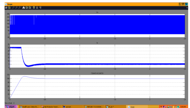
Figure 8: Simulink response of PID controller for torque T_L = 5 Nm and speed 100 rad/sec
