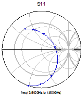
Figure 5: Smith Chart
