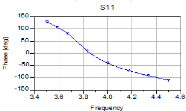
Figure 6: S parameter Display of S shape slotted microstrip patch antenna.
