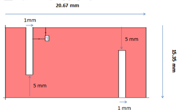
Figure 3: S- Slotted Microstrip Patch Antenna.
