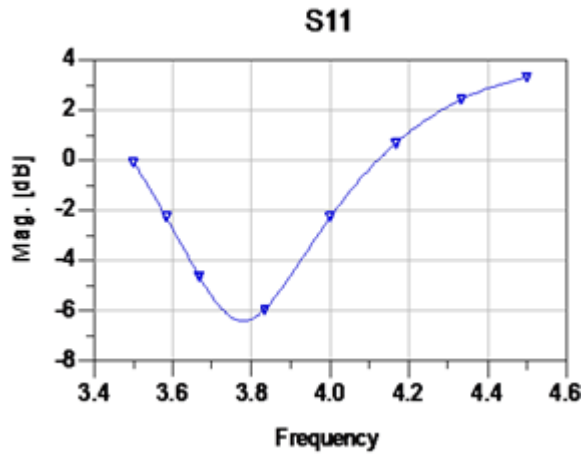
Figure 4: Reflection Coefficient of rectangular microstrip patch antenna
