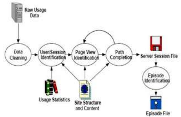
Figure 1: Preprocessing of Web Usage Mining
