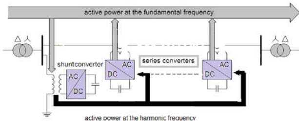
Figure 6: Active power exchange between DPFC converters
