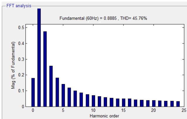
Figure 12: Total harmonic distortion of load voltage without DPFC
