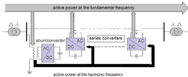
Figure 6: Active power exchange between DPFC converters
