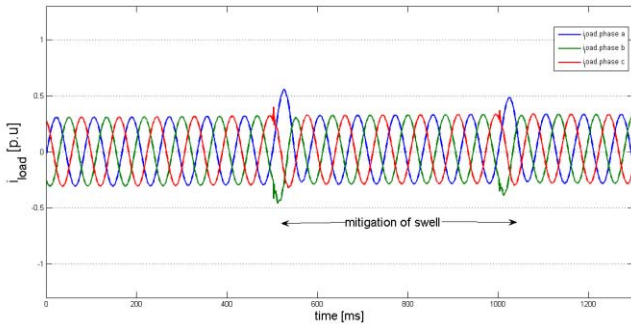
Figure 11: Mitigation of three-phase load current swell with DPFC
