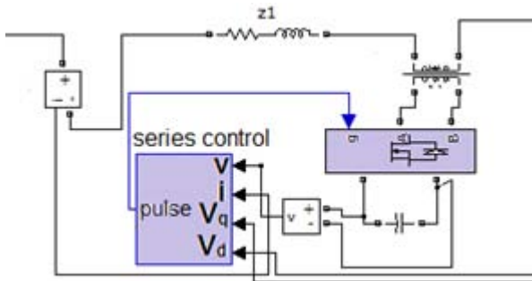
Figure 3: Block diagram of the series converters in Matlab/Simulink
