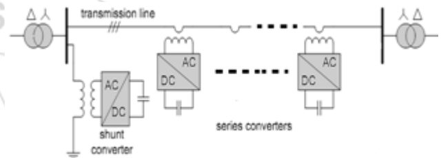
Figure 1: The DPFC Structure
