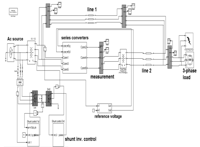
Figure 7: Simulation model of the DPFC
