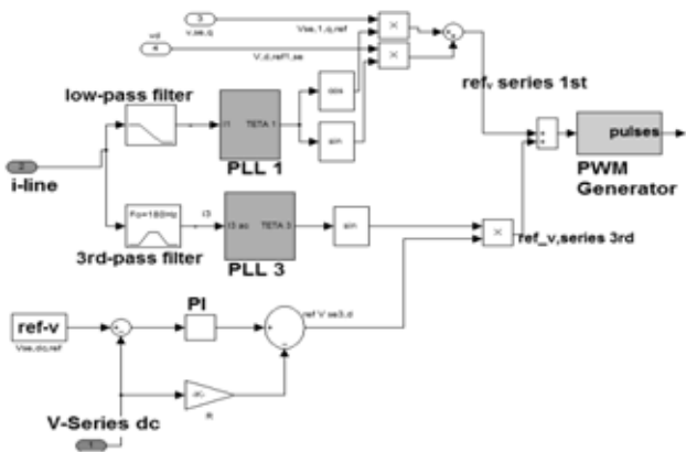
Figure 4: Block diagram of series control structure in Matlab/Simulink
