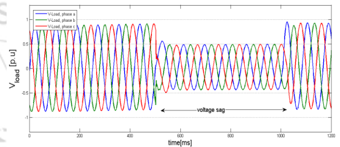
Figure 8: Three-phase load voltage sag waveform
