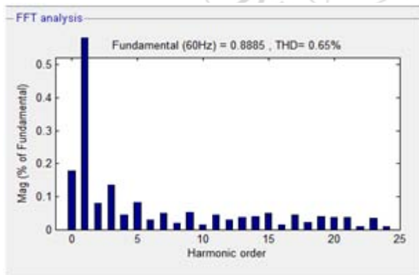
Figure 3: Total harmonic distortion of load voltage with DPFC
