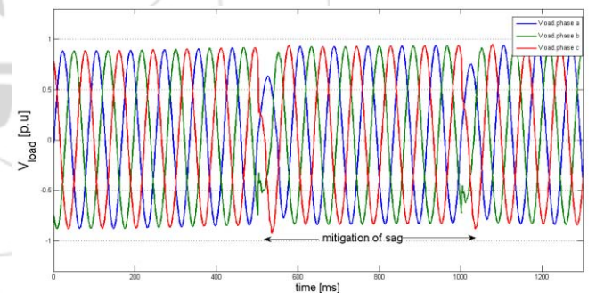
Figure 9: Mitigation of three-phase load voltage sag with DPFC
