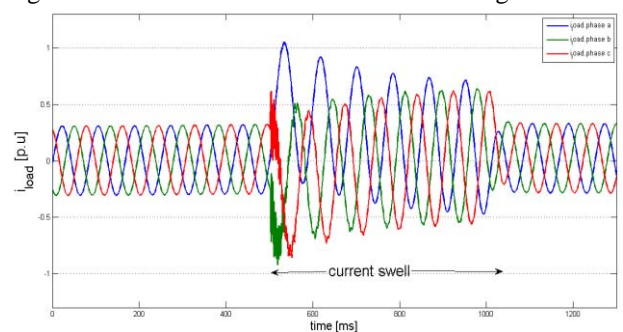
Figure 10: Three-phase load current swell waveform without DPFC
