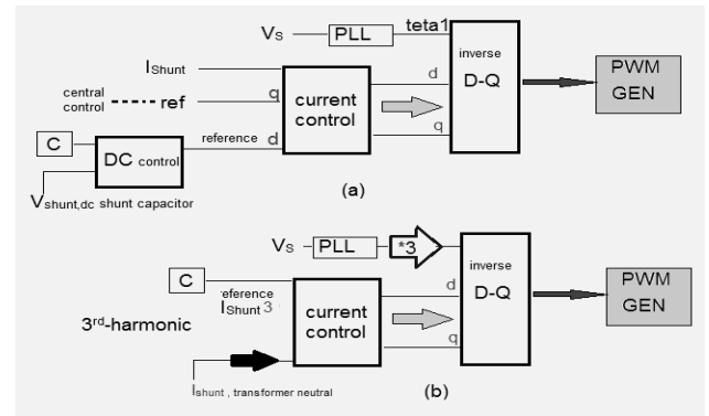
Figure 5: The shunt control configuration: (a) for fundamental frequency (b) for third-harmonic frequency
