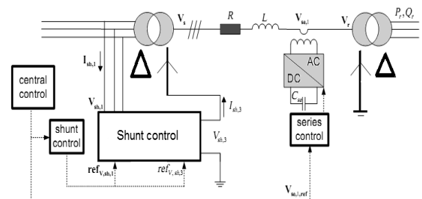
Figure 2: DPFC control structure
