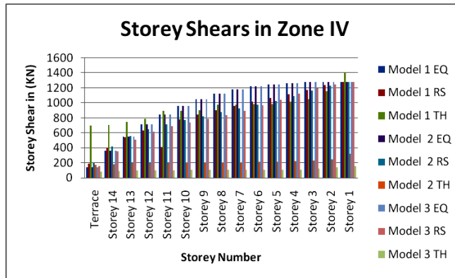
Chart 4: Showing Storey Shears in Zone IV
