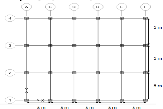
Figure 1: Showing the plan of a G+14 building
