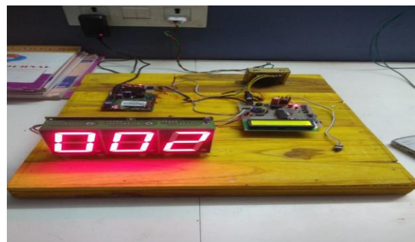
Figure 3: Displaying running Token number on 7 Segment display
