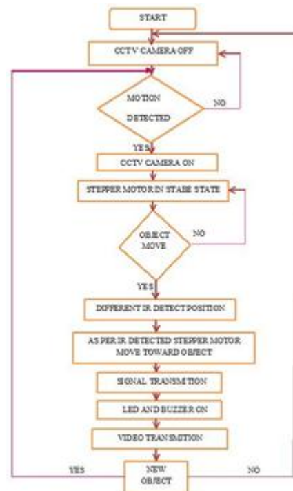
Figure 3: Flowchart of Automatic Mode
