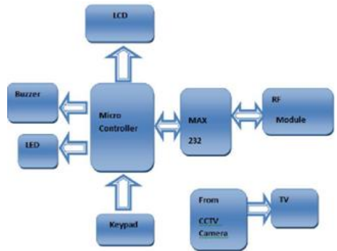
Figure 2: Control Unit
