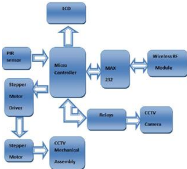
Figure 1: Surveillance Unit
