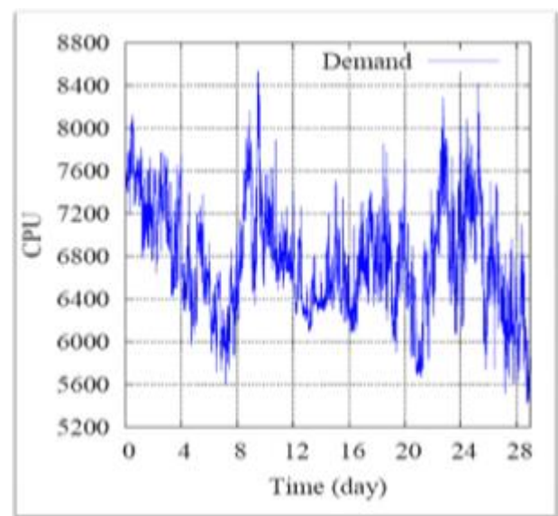
Figure: Total resource demand in Google's Cluster Data Set CPU Demand over 30 days
