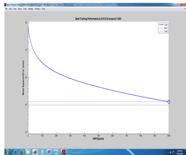
Figure 4: Simulation Result (Performance of IM)
