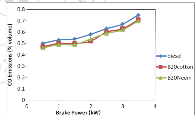
Figure 6: The variation of CO emissions with brake power
