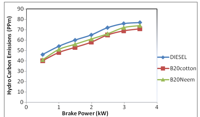
Figure 5: The variation of HC emissions with brake power
