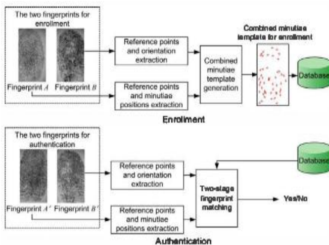
Figure 1: Phases of minutiae based algorithm
