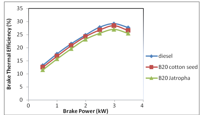
Figure 1: The variation of Brake thermal efficiency
