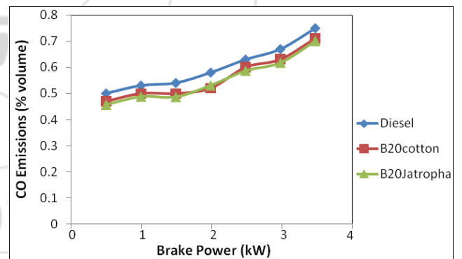
Figure 6: The variation of CO emissions with brake power
