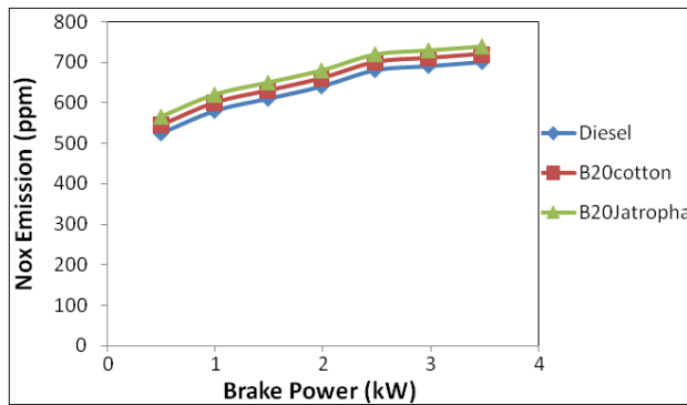
Figure 7: The variation of Nitrogen oxide emissions
