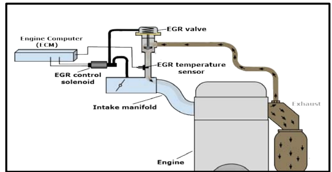
Figure 4: EGR System
