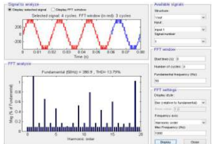
Figure 5.2.1: FFT plot of 9-level output voltage waveform of CMLI (without filter) [THD = 13.79%]
