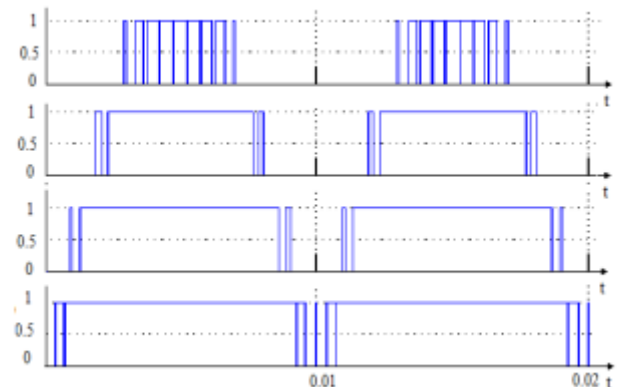
Figure 2.2: Gate signal for 9-level using PODPWM technique
