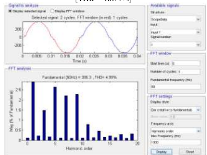
Figure 5.2.2: FFT plot of 9-level output voltage waveform of CMLI (with filter) [THD = 4.39%]
