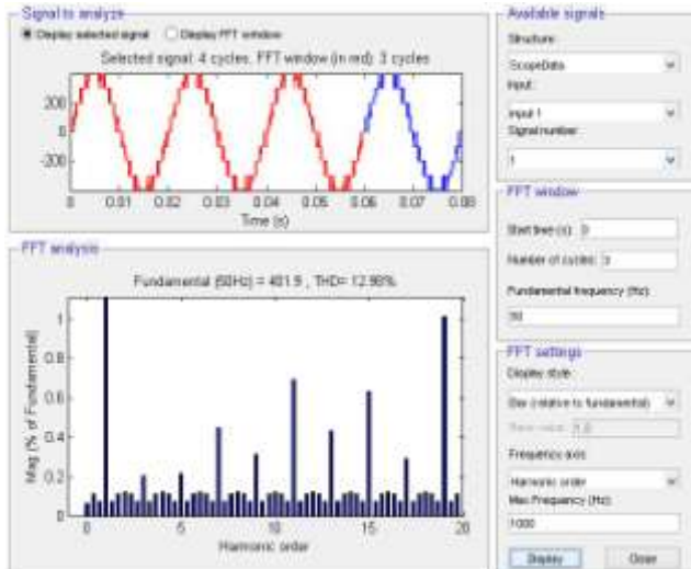
Figure 5.3.2: FFT plot of 9-level output voltage waveform of CMLI (without filter) [THD = 12.98%]
