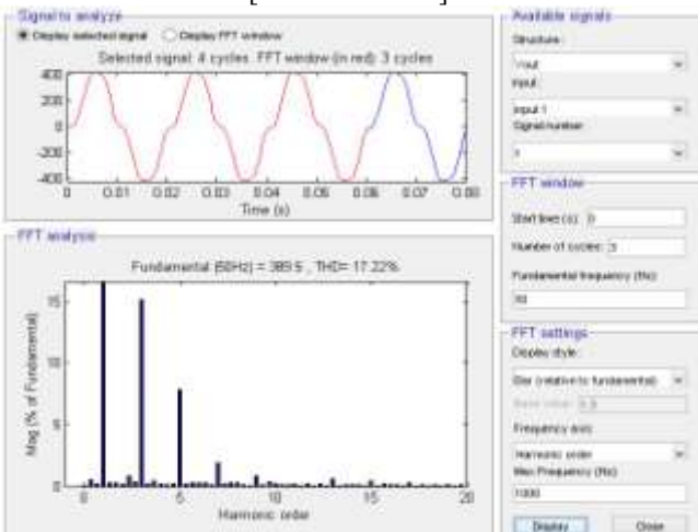
Figure 5.1.1: FFT plot of 9-level output voltage waveform of CMLI (with filter) [THD = 17.22%]
