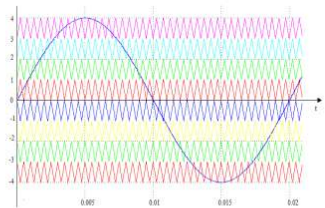
Figure 2.1: Carrier arrangement for PODPWM
