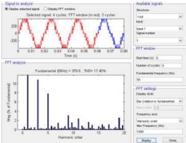
Figure 5.1.1: FFT plot of 9-level output voltage waveform of CMLI (without filter) [THD = 17.40%]
