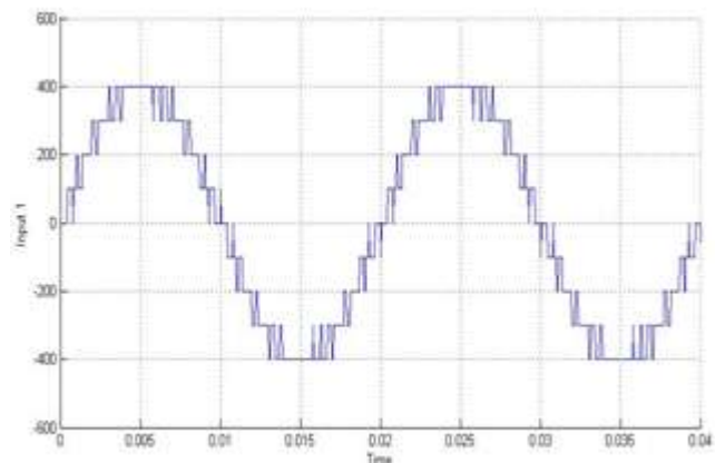
Figure 5.3.1: Simulated 9-level output voltage waveform of CMLI (without filter) using Modified PODPWM
