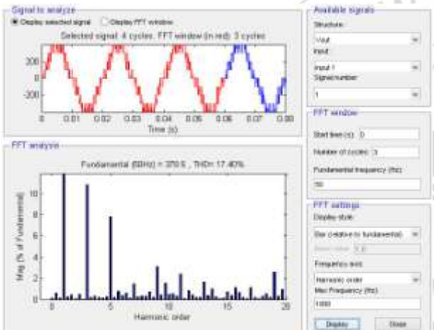
Figure 5.1.1: FFT plot of 9-level output voltage waveform of CMLI (without filter) [THD = 17.40%]
