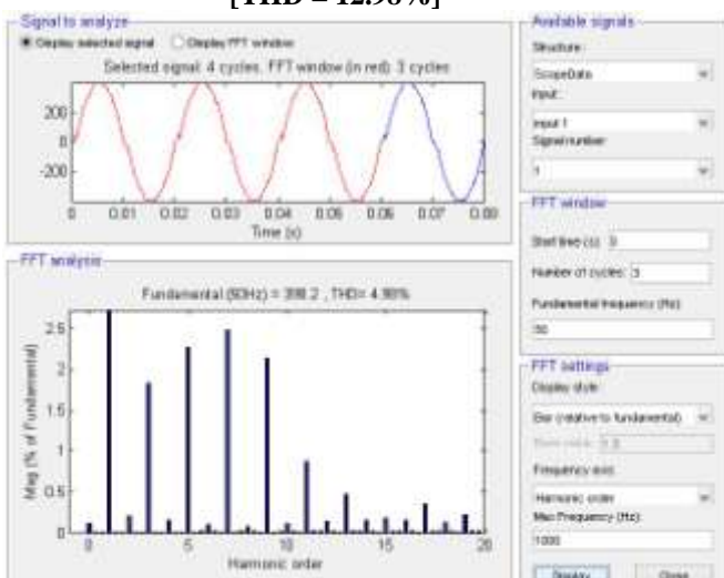
Figure 5.3.3: FFT plot of 9-level output voltage waveform of CMLI (with filter) [THD = 4.98%]
