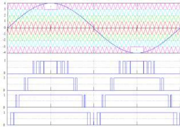
Figure 2.3: Modified PODPWM
