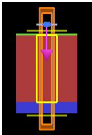
Figure 3: View of a: Si unit solar cell in FDTD Analysis
