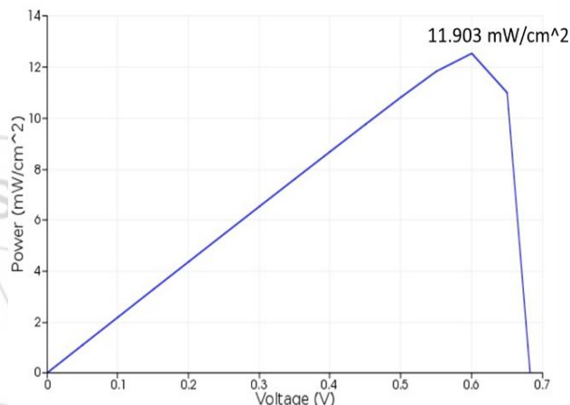
Figure 9(b): P-V characteristics with AR
