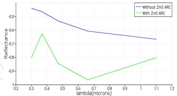
Figure 5: Reflectance of a:Si
