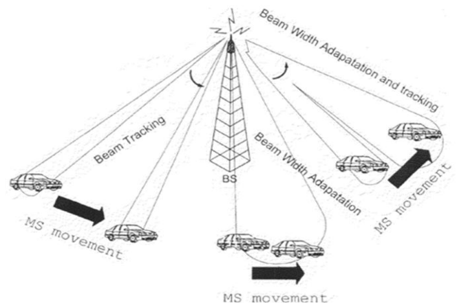
Figure 5: BDMA
