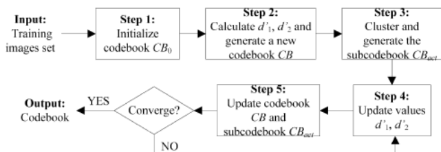
Figure 6: Codebooks generation algorithm
