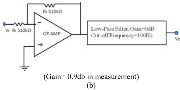
Fig. 1. (a) Active filter circuit with 80-dB 100-Hz cutoff frequency designed by TI FilterPro for the current sensor and (b) filter circuit designed for the voltage sensor with 0-dB 100-Hz cutoff frequency. The inverter is connected to the voltage sensor for providing a current path to virtual ground. sensor tag is accomplished by cutting the whole PET into pieces of the tags. Using fourth order Butterworth low-pass filter functioning as a low-pass active filter to in reduction circuitry will give better results.
