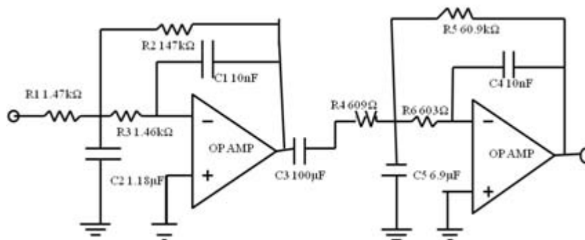
(Gain= 79.5db in measurement) (a)
