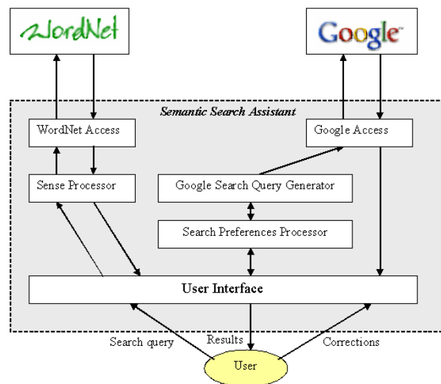
Figure 1: Semantic Search Engine Works
