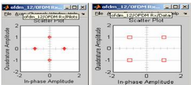
Figure 2 (a): ideal response of pilot tones and RX.
