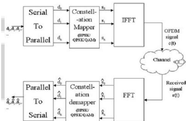
Figure 1: Block diagram of OFDM
