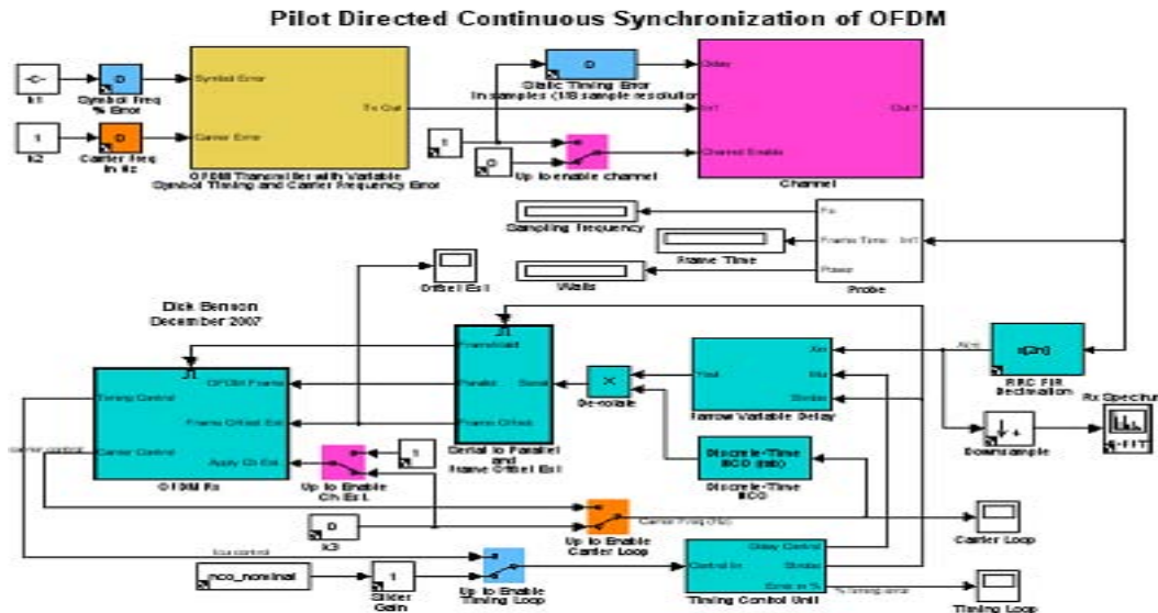
Figure 2: Pilot directed continuous synchronization of OFDM
