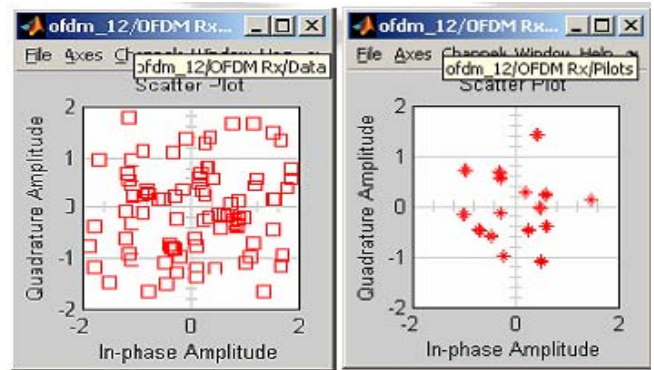
Figure 2 (b): Dispersive channel
