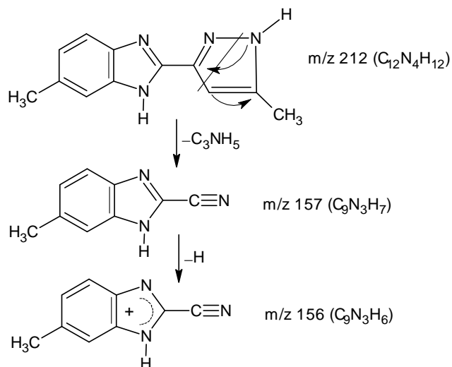
Figure 3: Fragmentation pathways with probable mechanisms from the mass spectrum of MBP.
