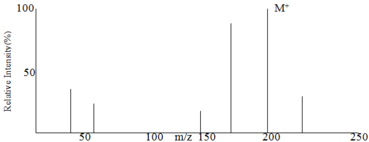
Figure (7.2) Mass Spectrum (0.70 eV) of 5-Methyl-3-(2,6-dimethylbenzimidazolyl) pyrazole
