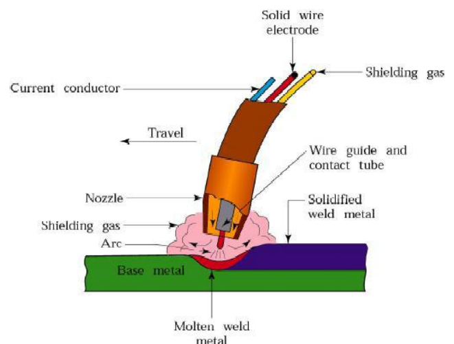
Figure 1.2: welding gun
