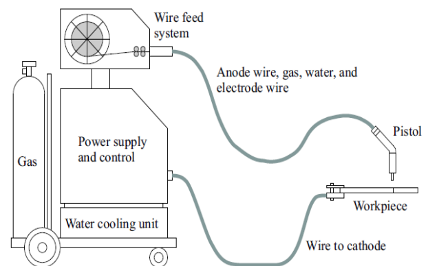
Figure 1: Typical gas metal arc welding setup
