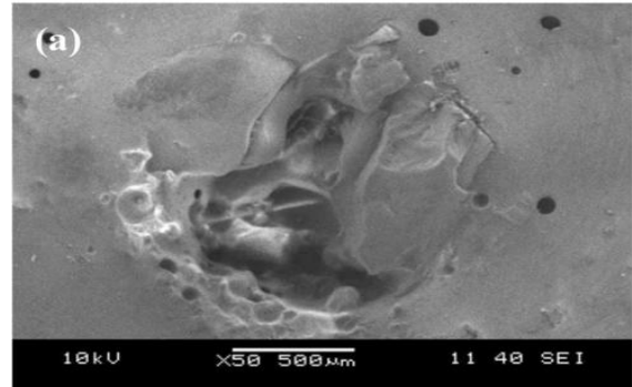
Figure 5.1: Microstructure of Parent Metal Martensitic stainless steel AISI 410
