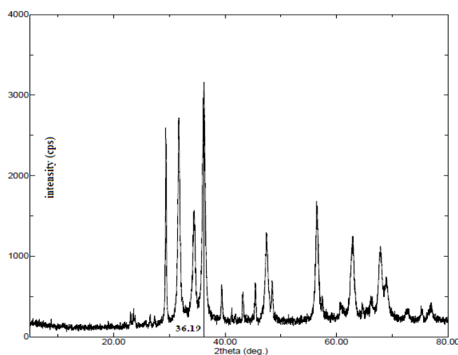
Figure 4: XRD pattern of Zinc Oxide nanoparticles
