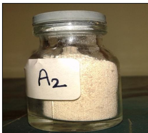
Figure 3: ZnO Nanoparticles
