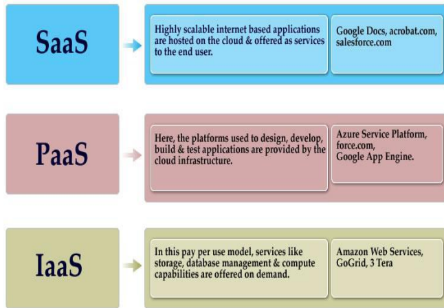
Figure 2: Cloud Models
