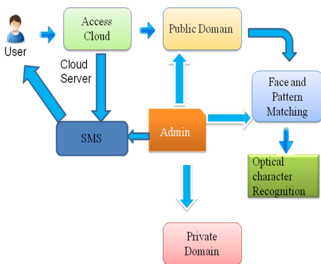
Figure 3: System Architecture
