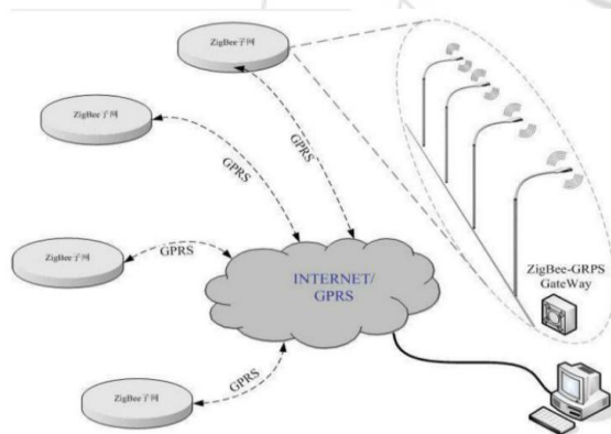
Figure 1: Proposed system View
