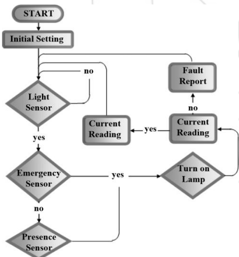
Figure 3: Control software flowchart
