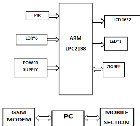
Figure 2: Proposed system Block Diagram
