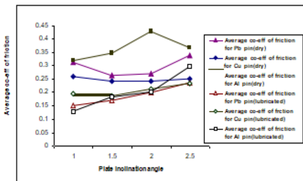
Figure 8 (a): The dependence of Average co-efficient of friction with plate inclination angle when Pb, Cu and Al pins slid on ground (SiC) steel surfaces
