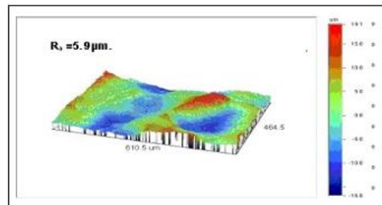
Figure 3 (b): The three- dimensional view of shot blast plate surface
