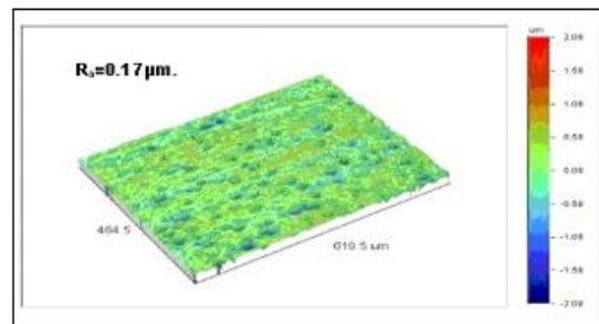
Figure 3 (a): The three- dimensional view of ground (SiC wheel polished) plate surface
