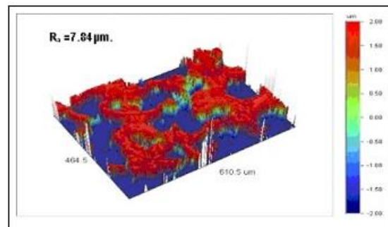
Figure 3 (c): The three- dimensional view of EDM plate surface
