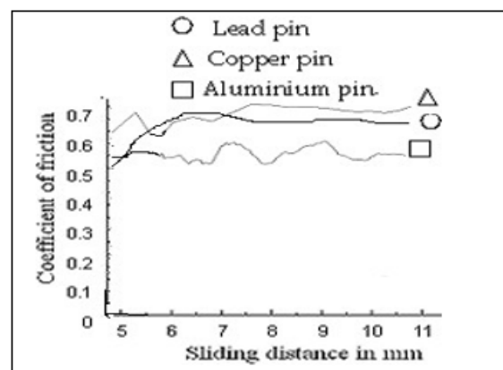
Figure 7: Dependency of co - efficient of friction with sliding distance for EDM steel surface.
