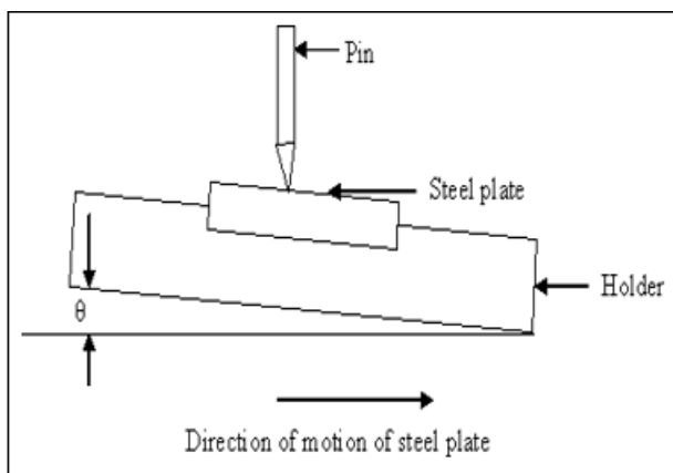
Figure 4: Schematic diagram of Pin on Plate with Inclined steel plate.
