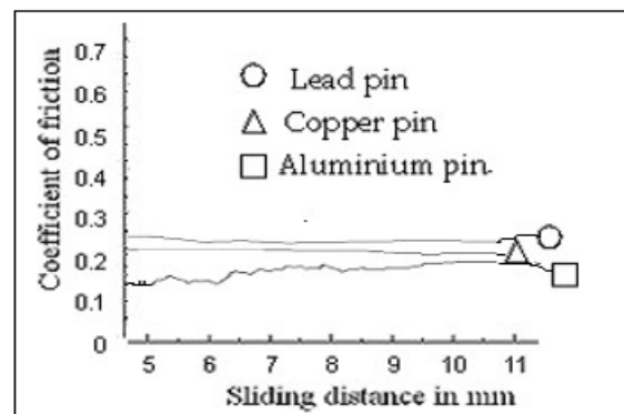
Figure 6: Dependency of co - efficient of friction with sliding distance for shot blast steel surface.
