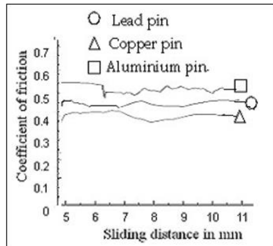
Figure 5: Dependency of co - efficient of friction with sliding distance for ground (SiC polished) steel surface.
