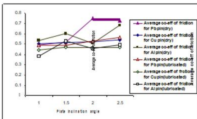
Figure 8 (c): The dependence of Average co-efficient of friction with plate inclination angle when Pb, Cu and Al pins slid on electric discharge machined steel surfaces
