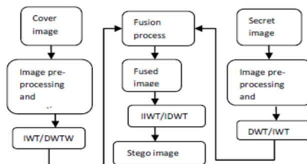
Figure 6: Existing Embedding Model
