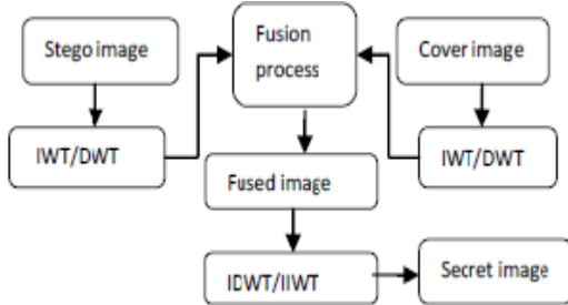
Figure 8: Based Extracting Model
