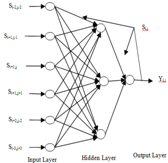
Figure 5: Feed Forward Neural Network
