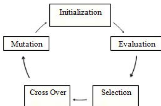
Figure 2: GA flow
