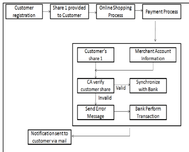
Fig. 2. Proposed Payment System.
