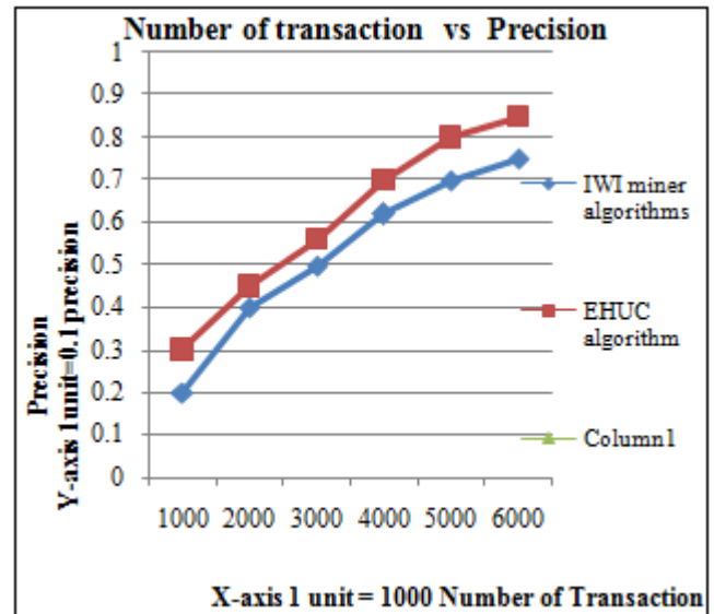
Figure 4: precision comparisons
