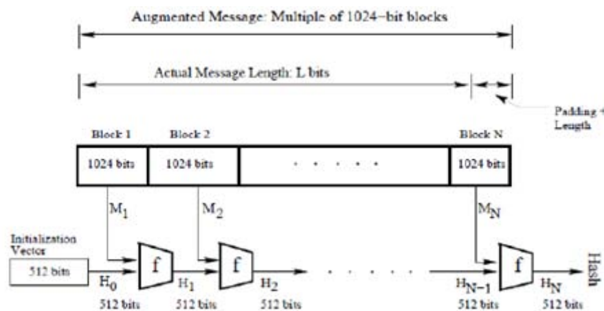
Figure 2: Overall Processing Steps of SHA 512
