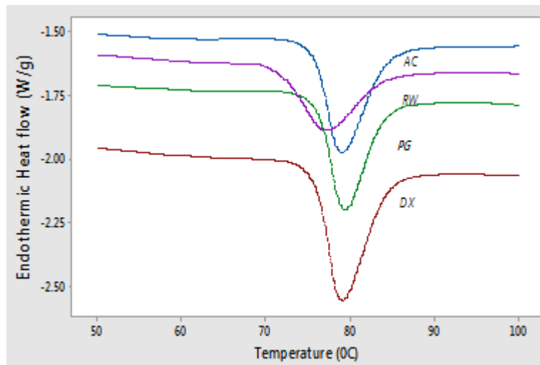
Figure 1: DSC thermograms of Native and modified Kithul flour
