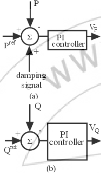
Figure 4.1: Series control scheme-automatic power flow mode
