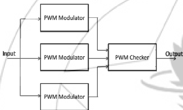
Figure 2: Triple Modular Redundancy
