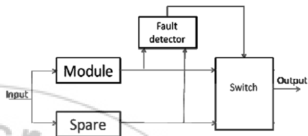
Figure 4: Standby Spare Arrangement
