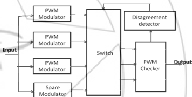
Figure 5: Block diagram of proposed system
